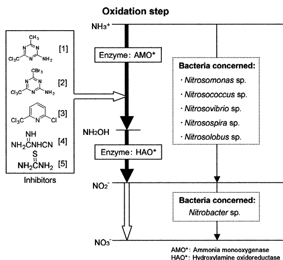
Fig. 2. Effect of inhibitors on nitrification of ammonia.
